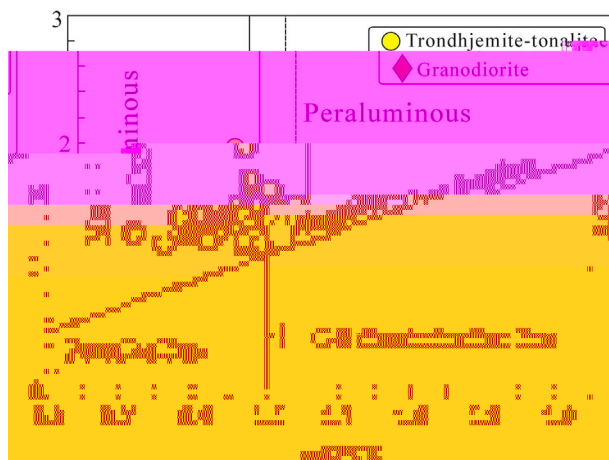
Fig. 7. ACNK vs. ANK diagram showing the metaluminous signature of the trondhjemite-tonalites and the granodiorite.
